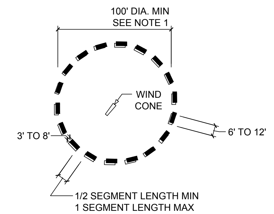
3 SEGMENTED CIRCLE MARKER AND WIND DIRECTION INDICATOR 1" = 1'-0"
