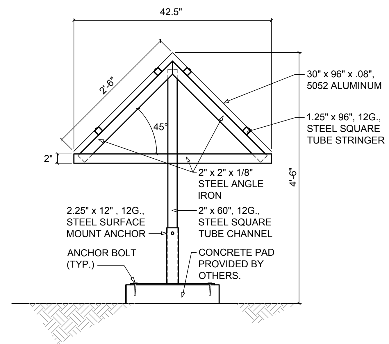
1 HB-5340 SEGMENTED CIRCLE SIDE VIEW 1" = 1'-0"
