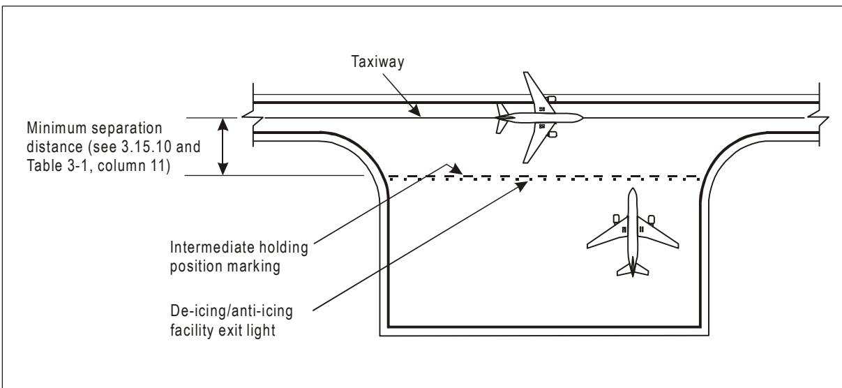
Figure 5-26. Typical remote de-icing/anti-icing facility
