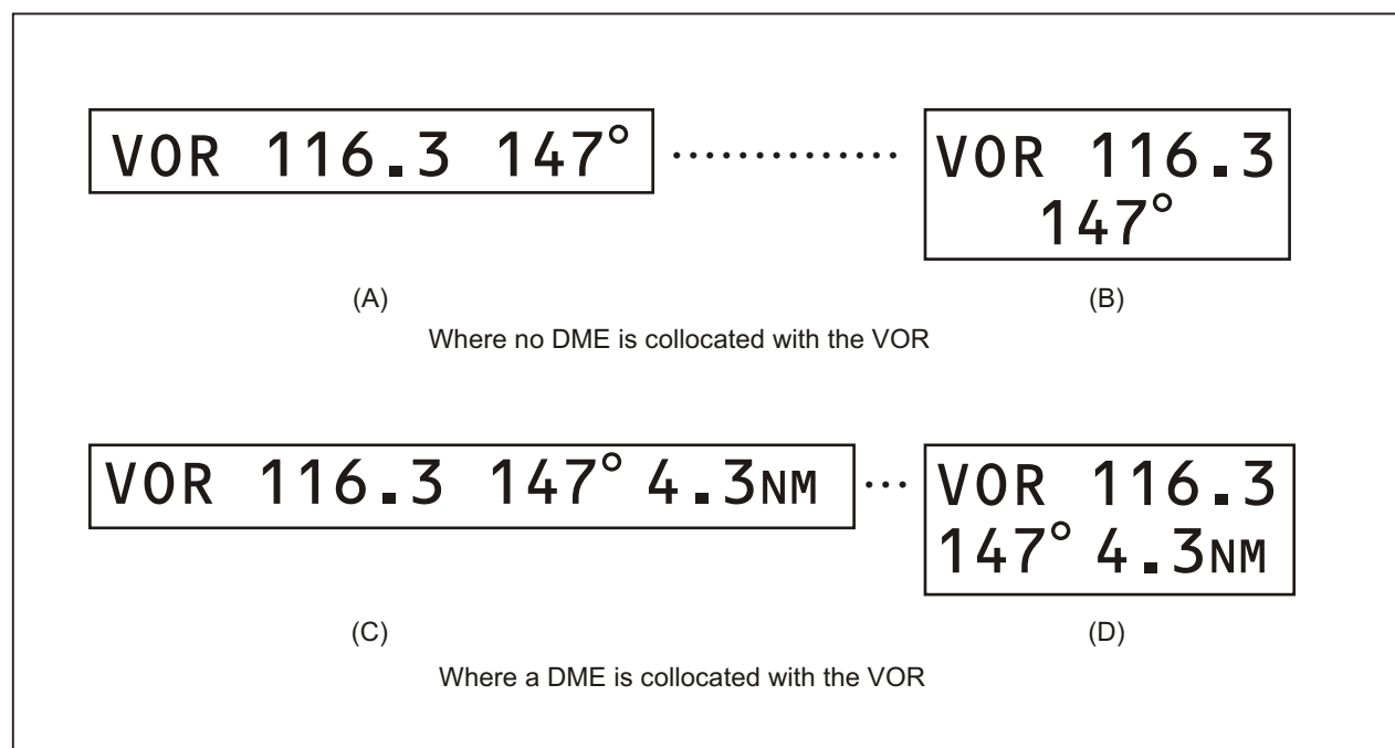
Figure 5-31. VOR aerodrome check-point sign
