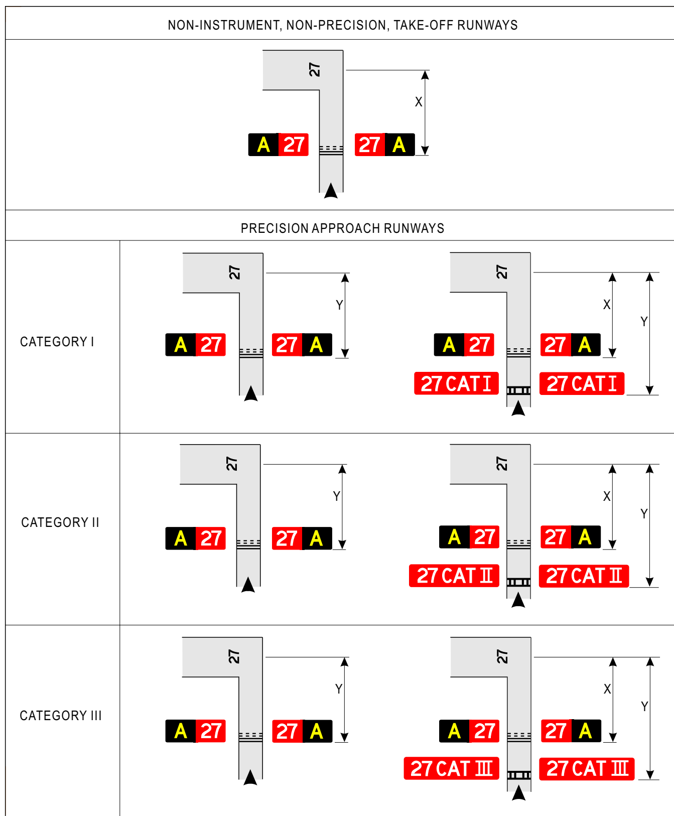
Figure 5-30. Examples of sign positions at taxiway/runway intersections
