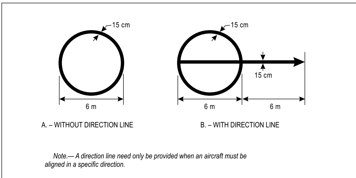
Figure 5-8. VOR aerodrome check-point marking
