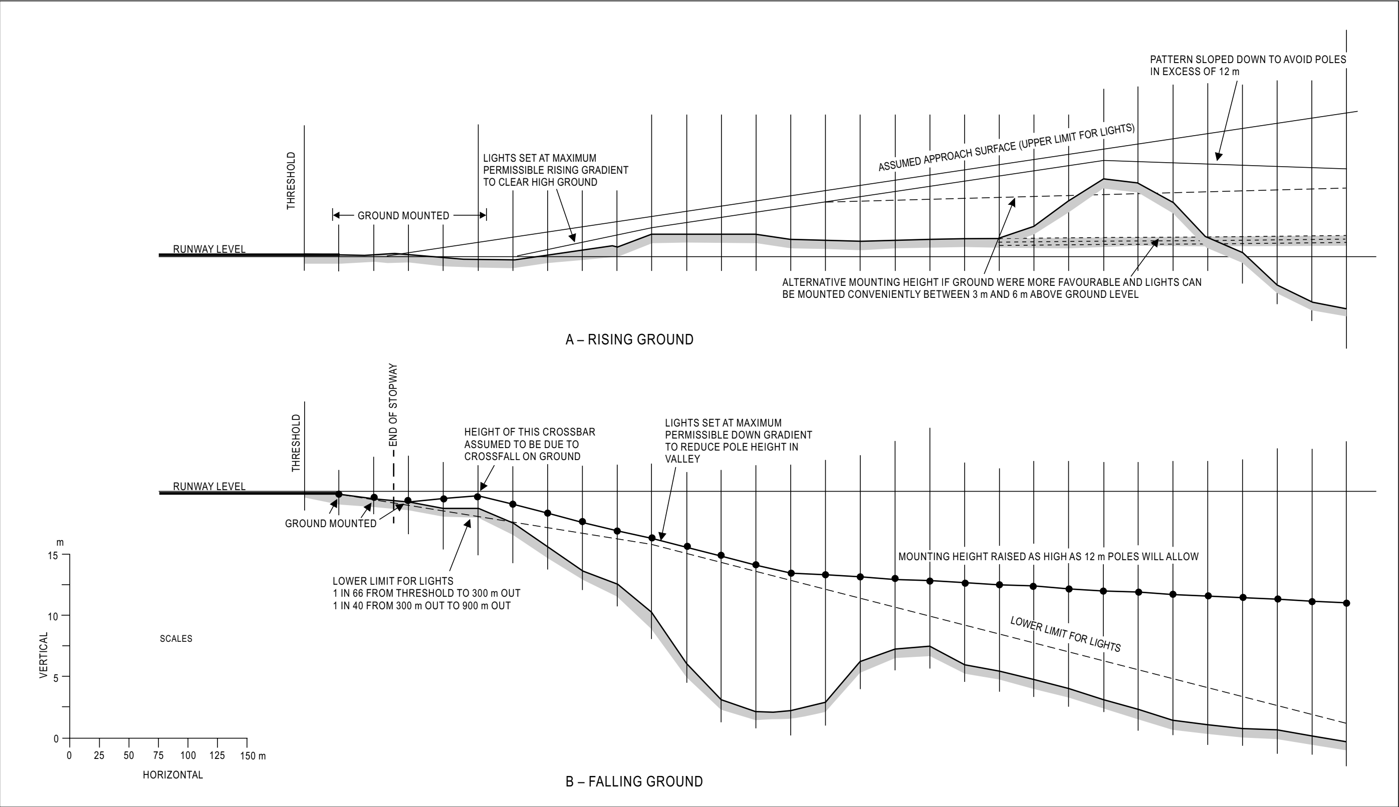
Figure A-7. Vertical installation tolerances
