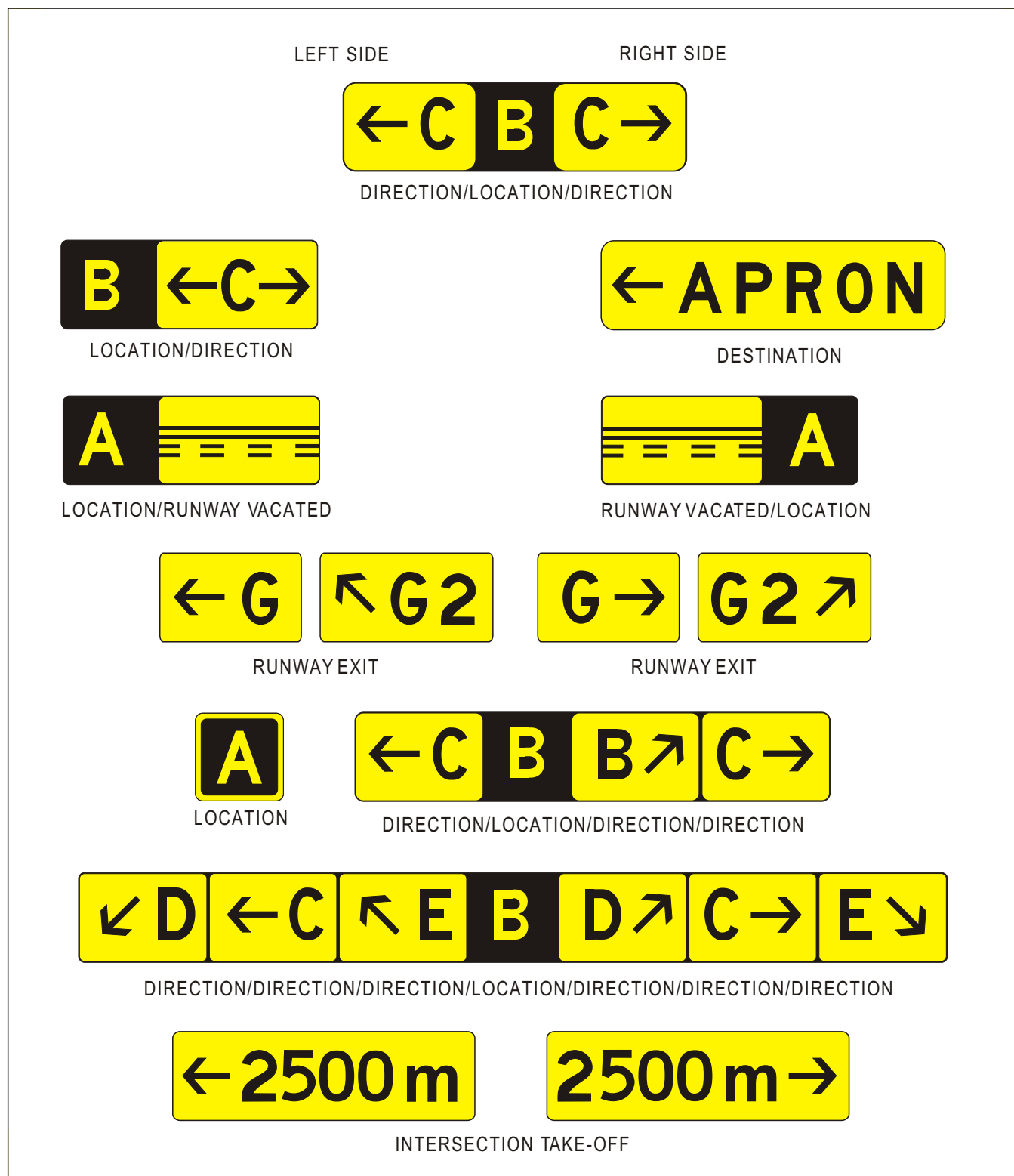
Figure 5-29. Information signs
