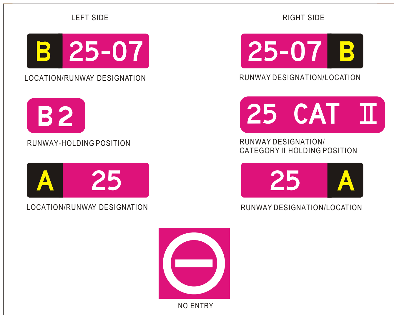
Figure 5-28. Mandatory instruction signs
