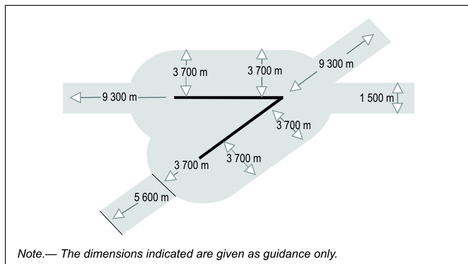
Figure 5-11. Multiple runway laser-beam free flight zone
