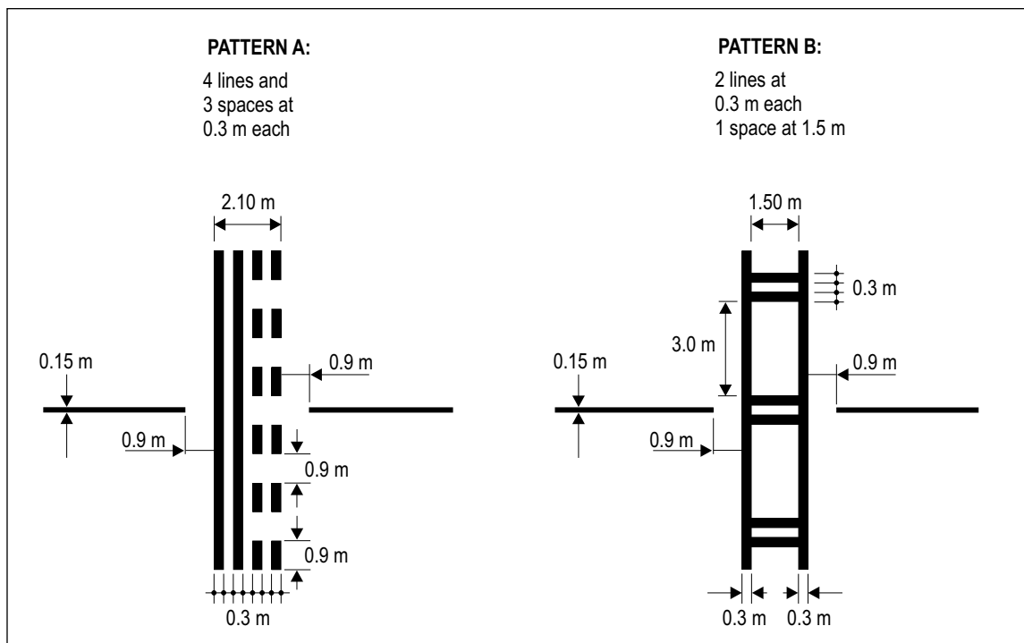
Figure 5-7. Runway-holding position markings
