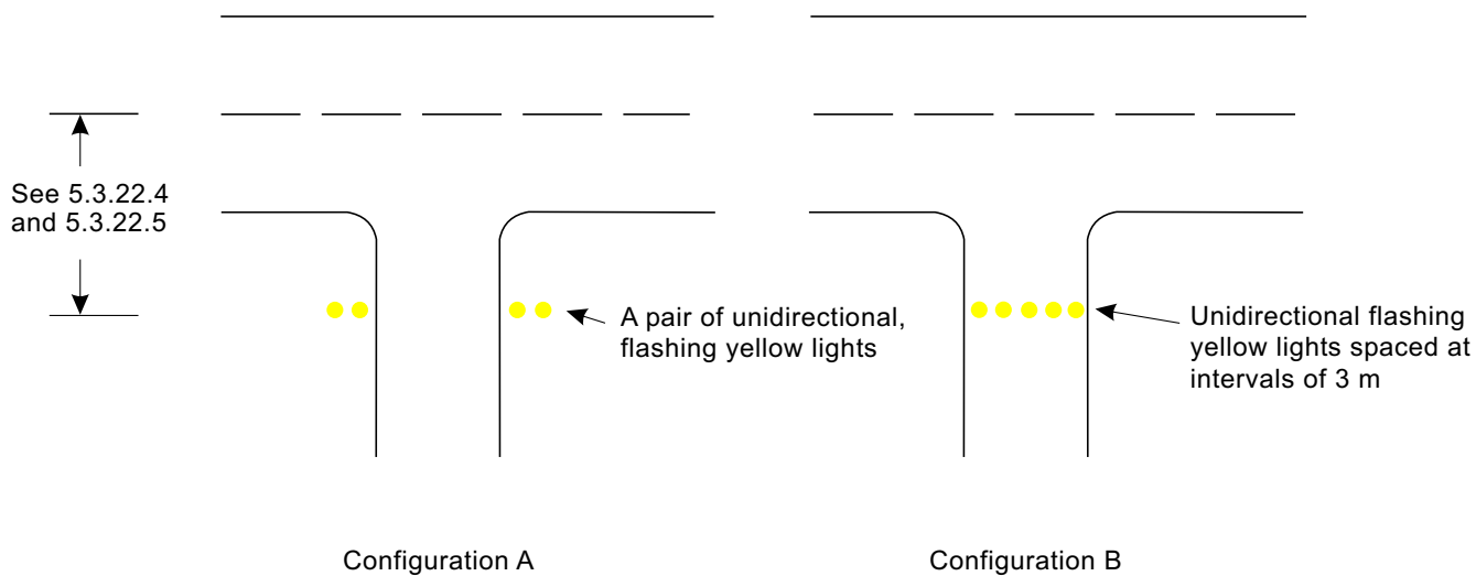
Figure 5-27. Runway guard lights
