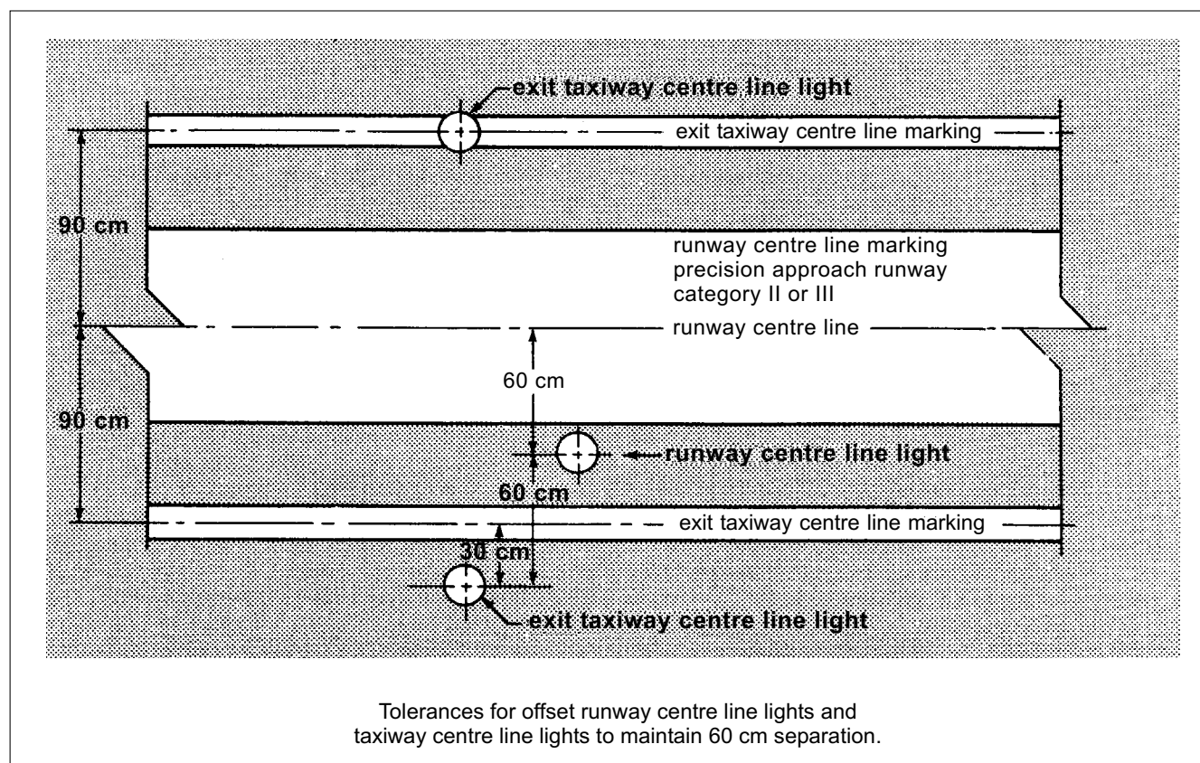
Figure 5-25. Offset runway and taxiway centre line lights
