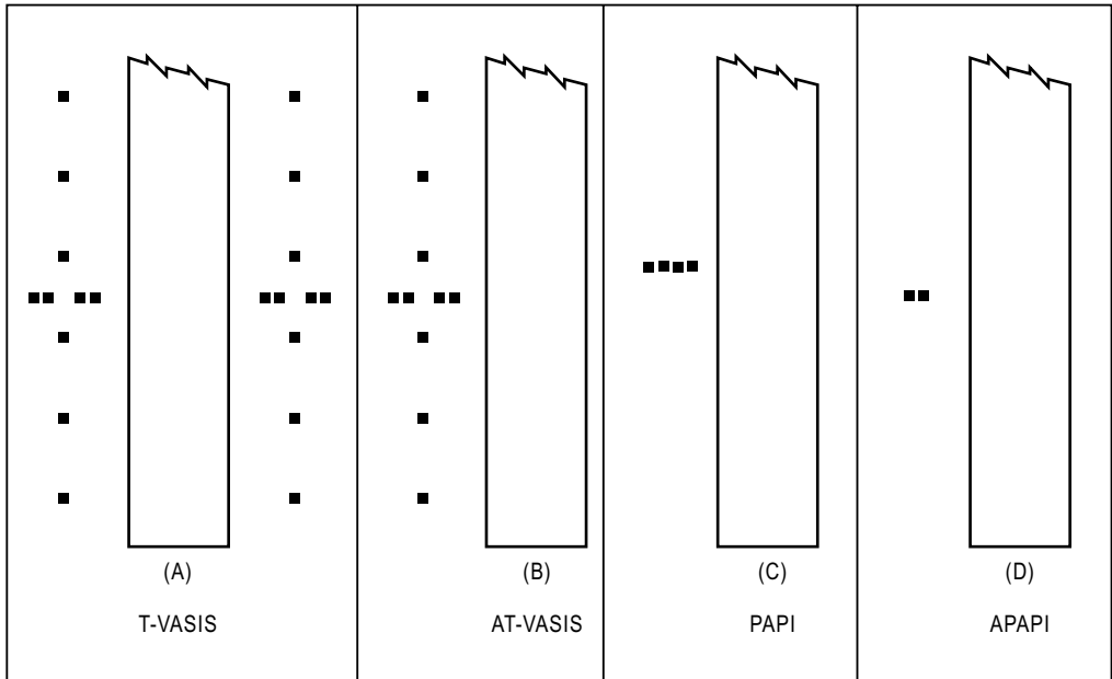
Figure 5-15. Visual approach slope indicator systems
