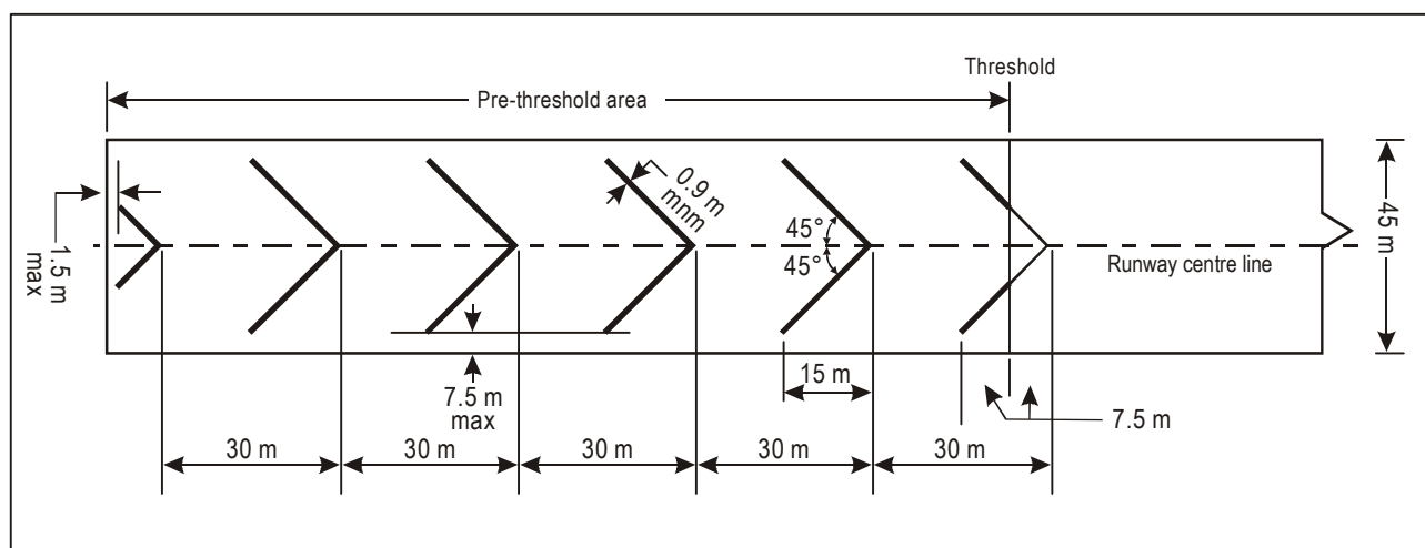
Figure 7-2. Pre-threshold marking
