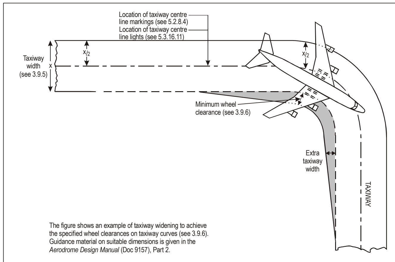
Figure 3-2. Taxiway curve
