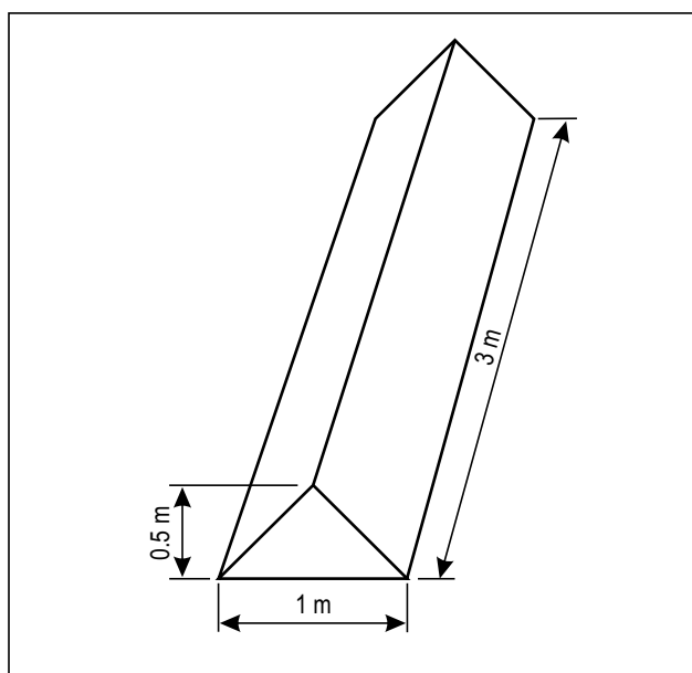
Figure 5-32. Boundary markers
