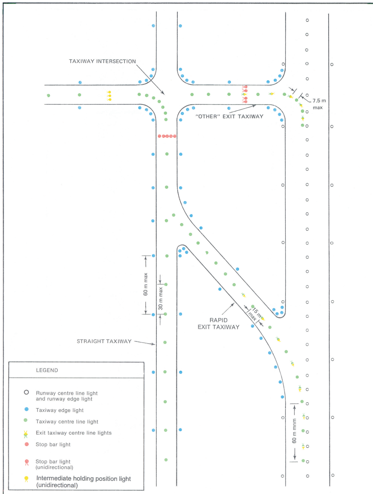
Figure 5-24. Taxiway lighting
