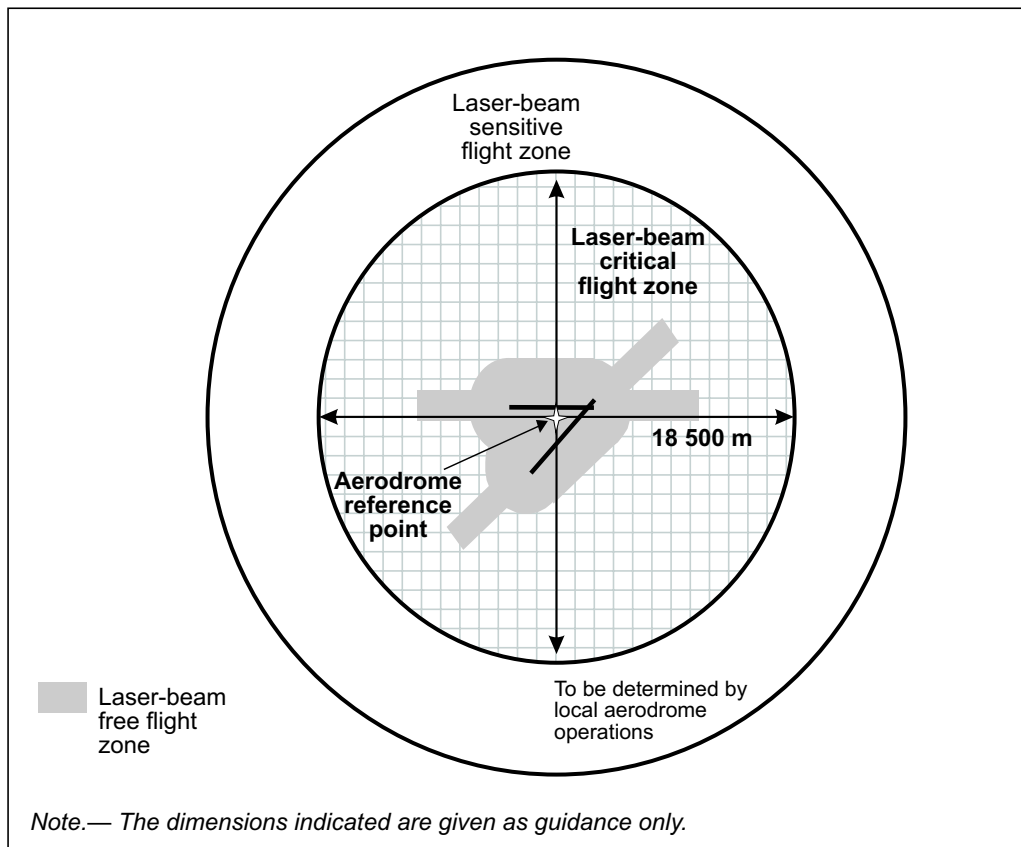
Figure 5-10. Protected flight zones
