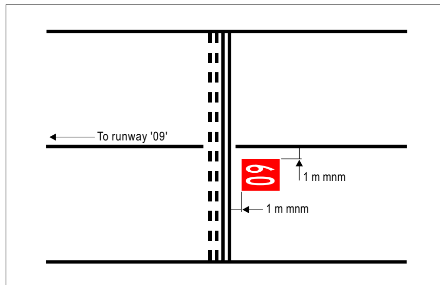
Figure 5-9. Mandatory instruction marking
