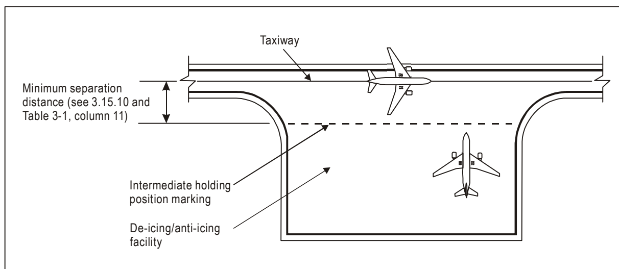
Figure 3-4. Minimum separation distance on a de-icing/anti-icing facility
