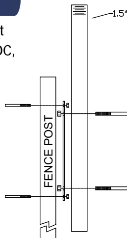
POST TO POST MOUNT
