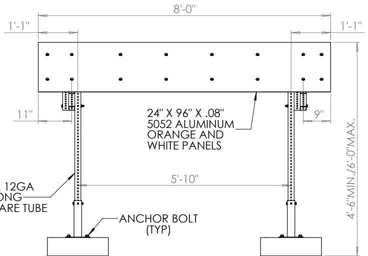
Hali-Brite® Model HB-5340-8-2S
